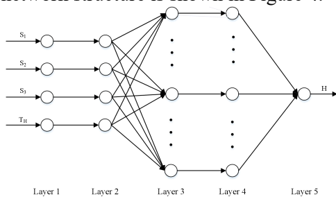
Figure 4. Fuzzy Neural Network Structure
