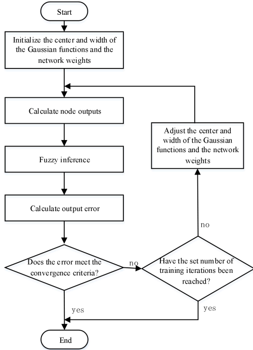
Figure 5. Fuzzy Neural Network Training Flow Chart
