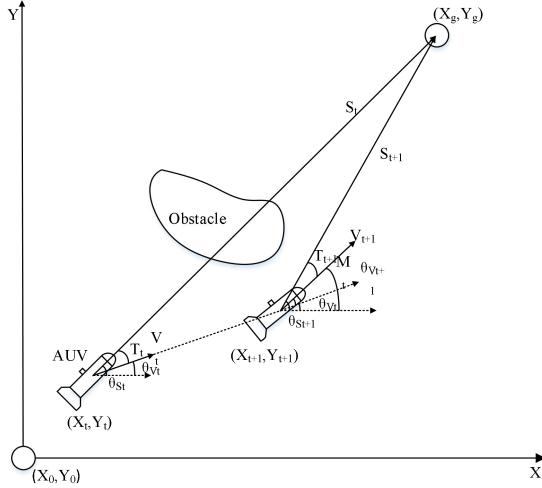
Figure 3. AUV Horizontal Obstacle Avoidance Model
